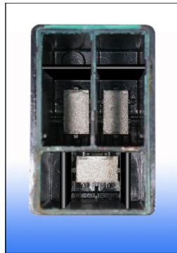
1a) Top view onto an opened HP342 cartridge.
