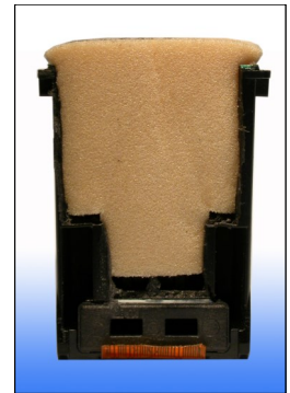
1c) Cross-section view of yellow ink chamber with sponge inserted.
