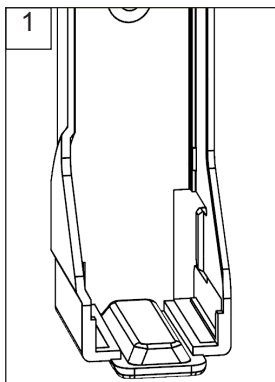
Install the seal in the center of the clip.
